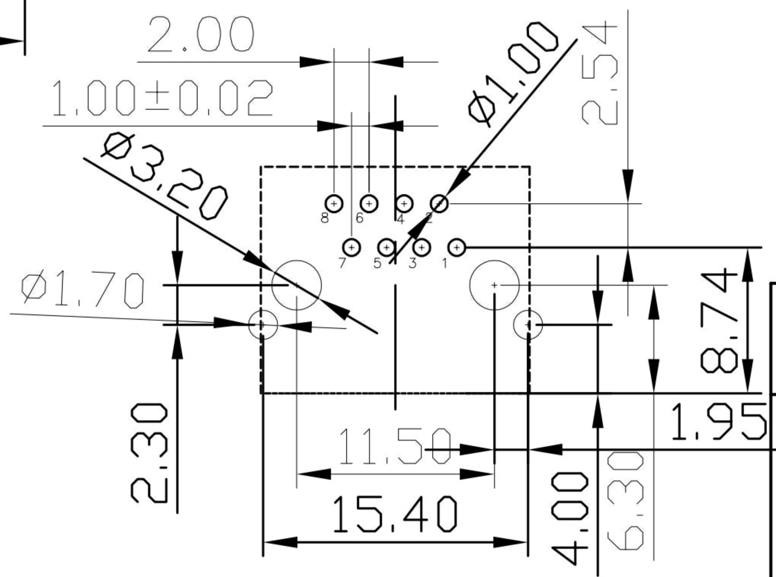
RECOMMENDED PCB LAYOUT TOP VIEW(TOL:±0.05)
