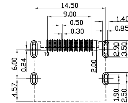
RECOMMEND PCB LAYOUT(±0.05)
