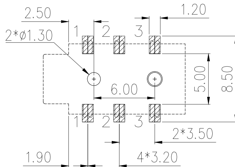
RECOMMEND PCB LAYOUT(±0.05)
