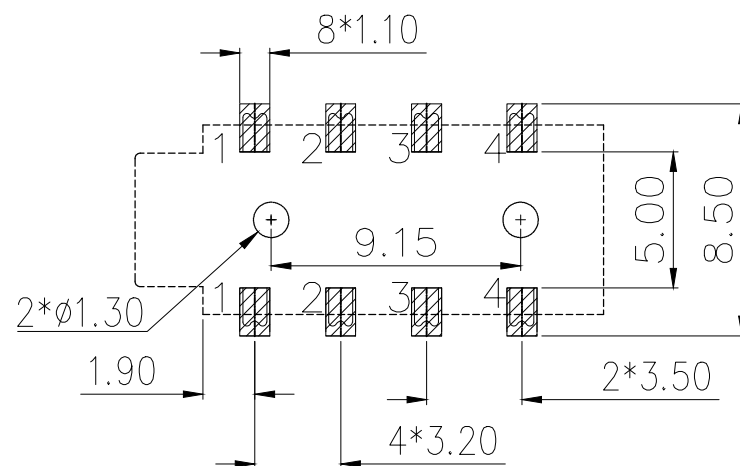
RECOMMEND PCB LAYOUT(±0.05)
