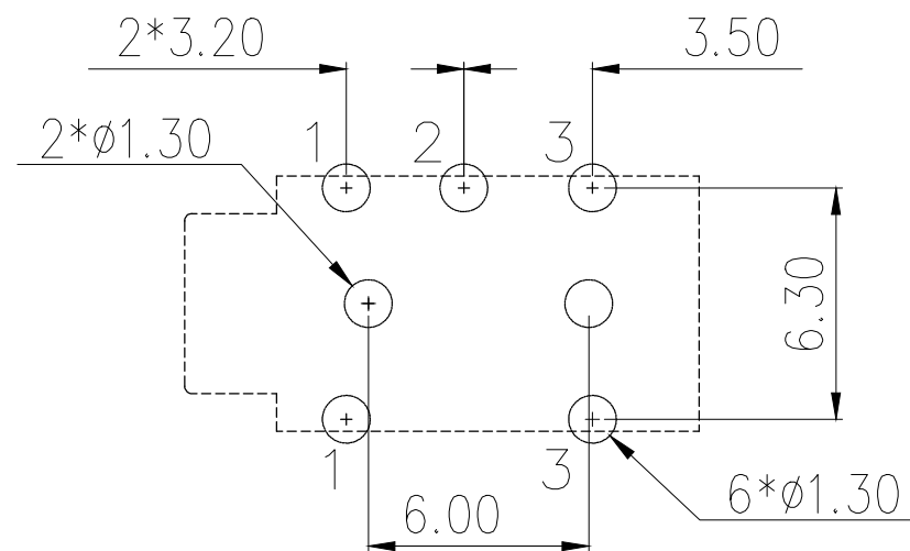
RECOMMEND PCB LAYOUT(±0.05)
