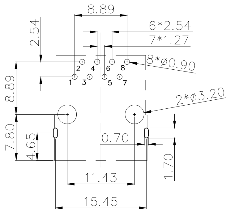
RECOMMENDED PCB LAYOUT TOP VIEW(TOL:±0.05)
