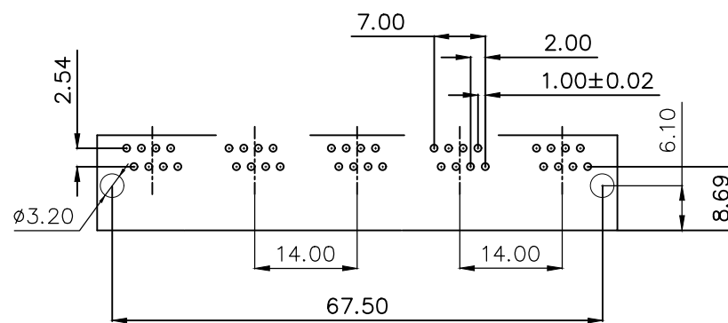
RECOMMENDED PCB LAYOUT TOP VIEW(TOL: \pm 0.05 )
