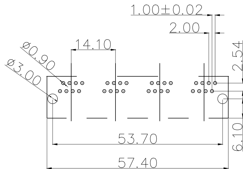
RECOMMENDED PCB LAYOUT TOP VIEW(TOL: ±0.05)
