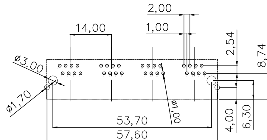
RECOMMENDED PCB LAYOUT TOP VIEW(TOL: ±0.05)
