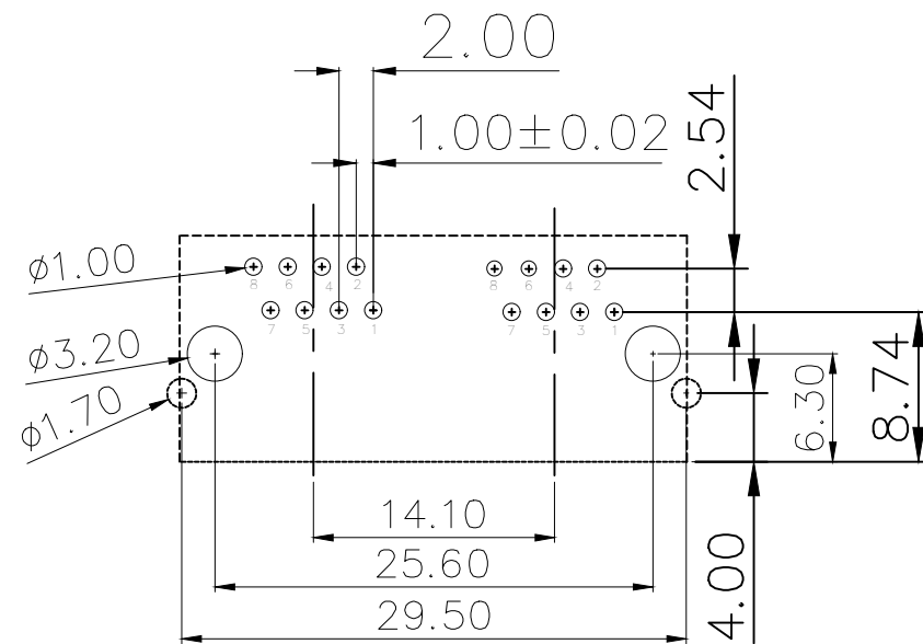
RECOMMENDED PCB LAYOUT TOP VIEW(TOL: \pm 0.05 )
