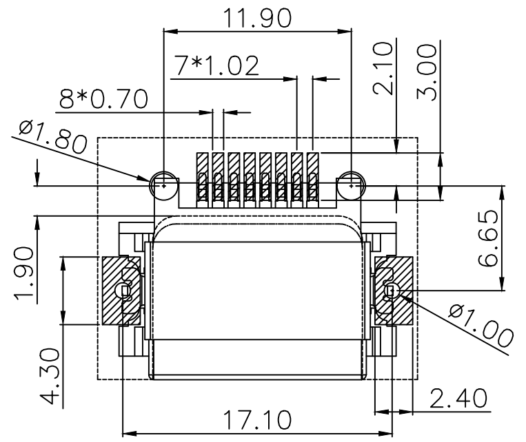
▨ PAD AREA (TOP VIEW)
