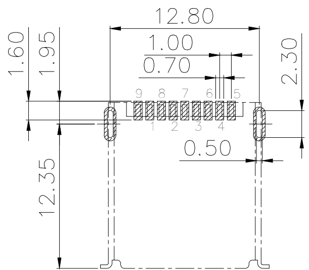
RECOMMEND PCB LAYOUT(±0.05)
