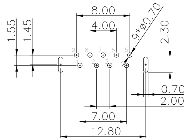
RECOMMENDER P.C.B.LAYOUT TOP VIEW (COMPONENT SIDE TOLERANCE±0.05)
