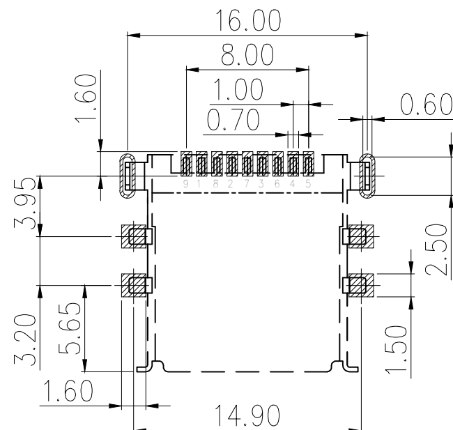
RECOMMEND PCB LAYOUT(±0.05)
